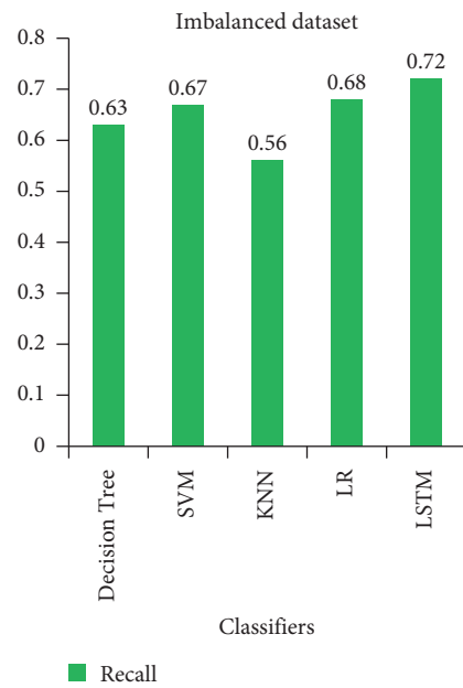
FIGURE 6: The recall value of imbalanced dataset.
