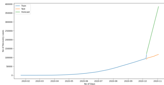
Figure 5 Recovery Cases forecasting using ES
