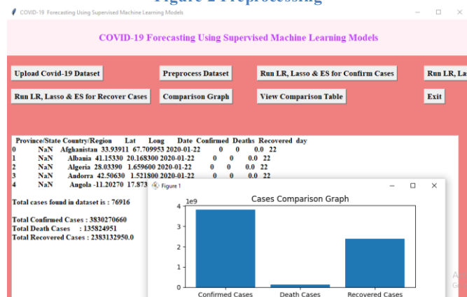
Figure 2 Preprocessing
