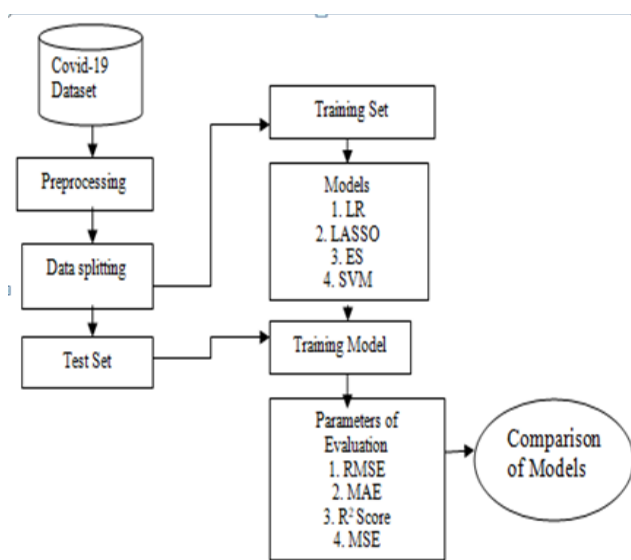
Figure 1 Proposed Workflow
