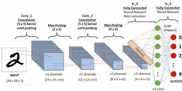
Fig.3. CNN Structure
